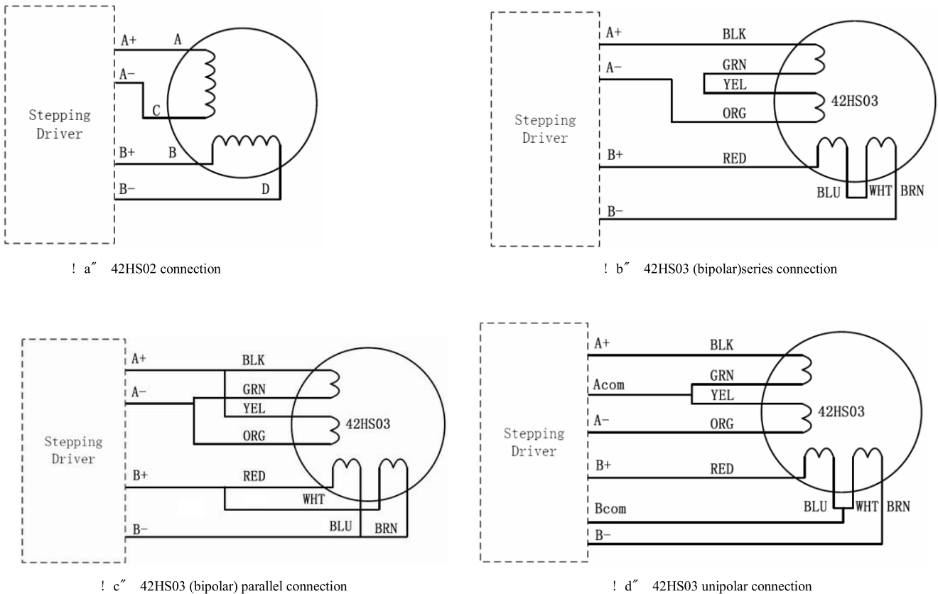
Figure 3: Wiring diagram
