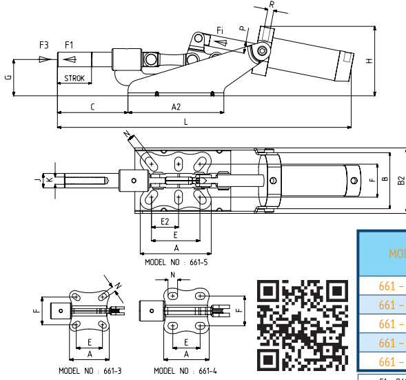
Body Mounting Base Horizontal With Welding, Tied Front
