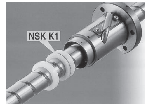
Fig. 3.29 Ball screws equipped with NSK K1™ lubrication units Page B577
