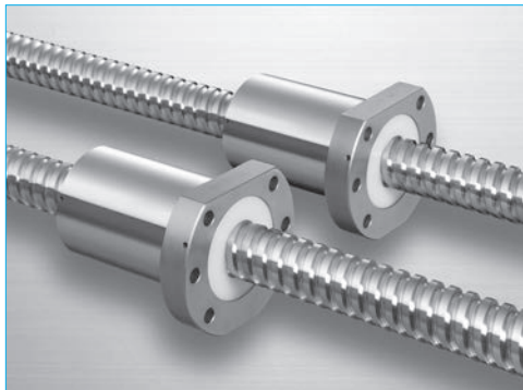
Fig. 3.23 TW series for twin-drive systems Page B543
