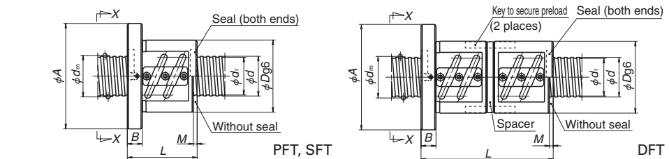
View X-X
