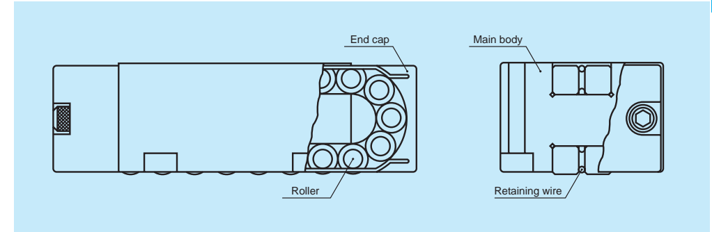
Fig. 1 Linear roller bearing
