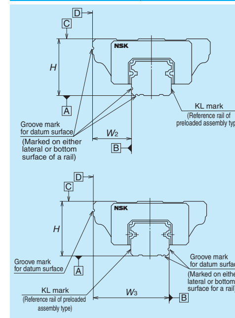
Fig. 4.1 Assembled dimensions
