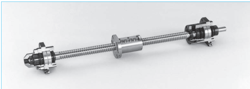
Fig. 3.25 Hollow shaft ball screws for high-precision machine tools Page B544
