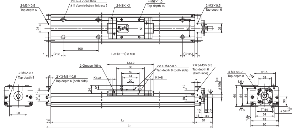
Dimension of MCM08 (Single slider)
