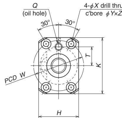
View X-X
