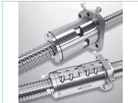
Fig. 3.24 Nut cooling ball screws for high precision machine tools Page B549
