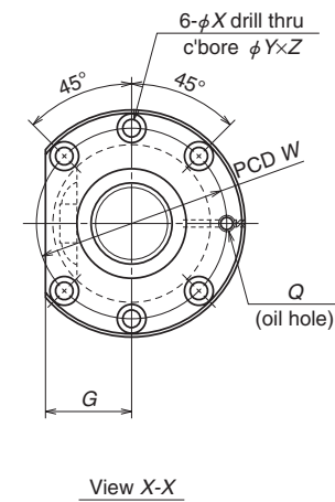
View X-X
