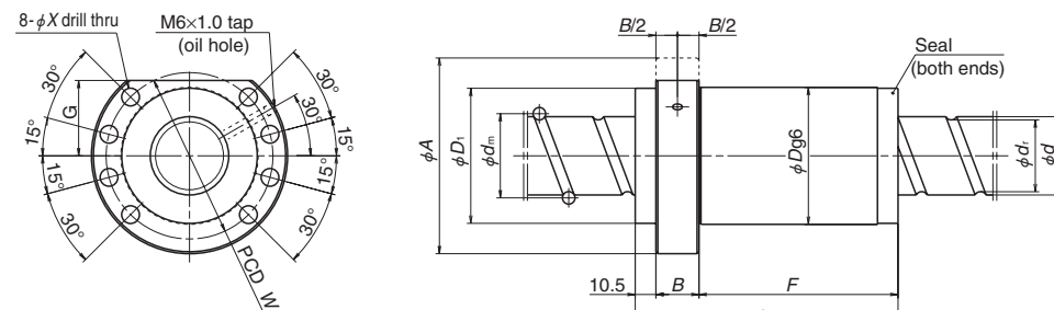
Screw shaft diameter d \geq 36 mm
