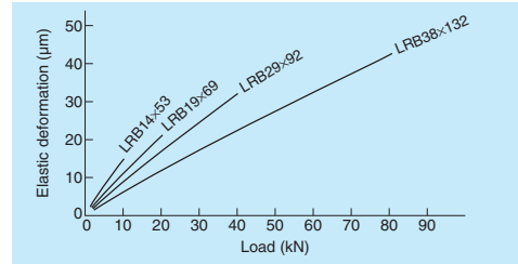
Fig. 2 Elastic deformation
