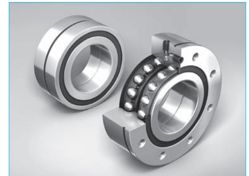
Fig. 3.40 Ball screw support bearings Page B425 BSBD series
