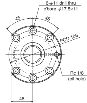
View X-X
