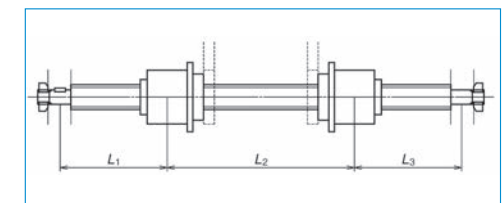
Fig. 4 Installation example
