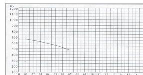
* Hardenability curve
