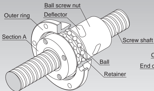
Structure of Standard-Lead Rotary Nut Ball Screw Model DIR
